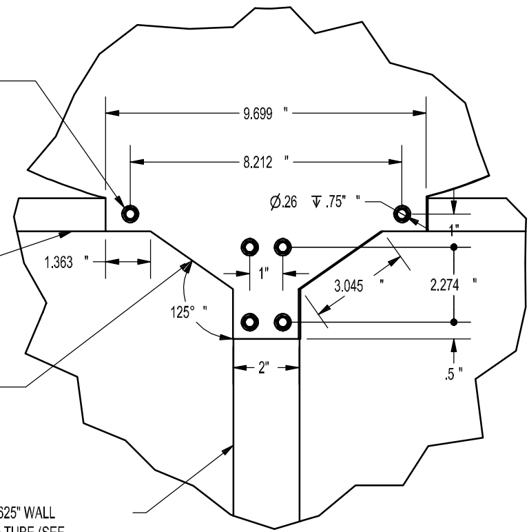
DETAIL B SCALE 1/4" = 1"
